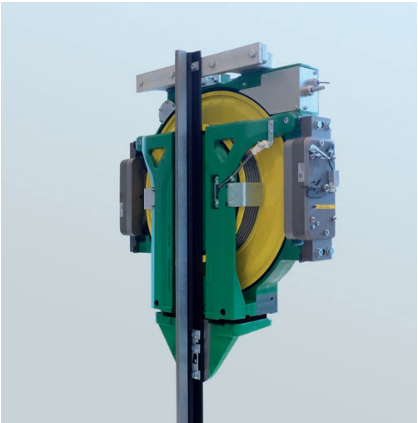
The eco-efficient KONE EcoDisc hoisting system
